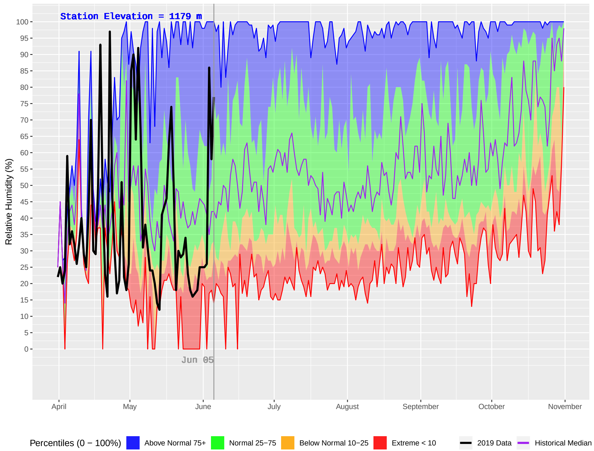
HOLMES (201) : Historical (1987–2018) and Current (2019) Daily Relative Humidity
