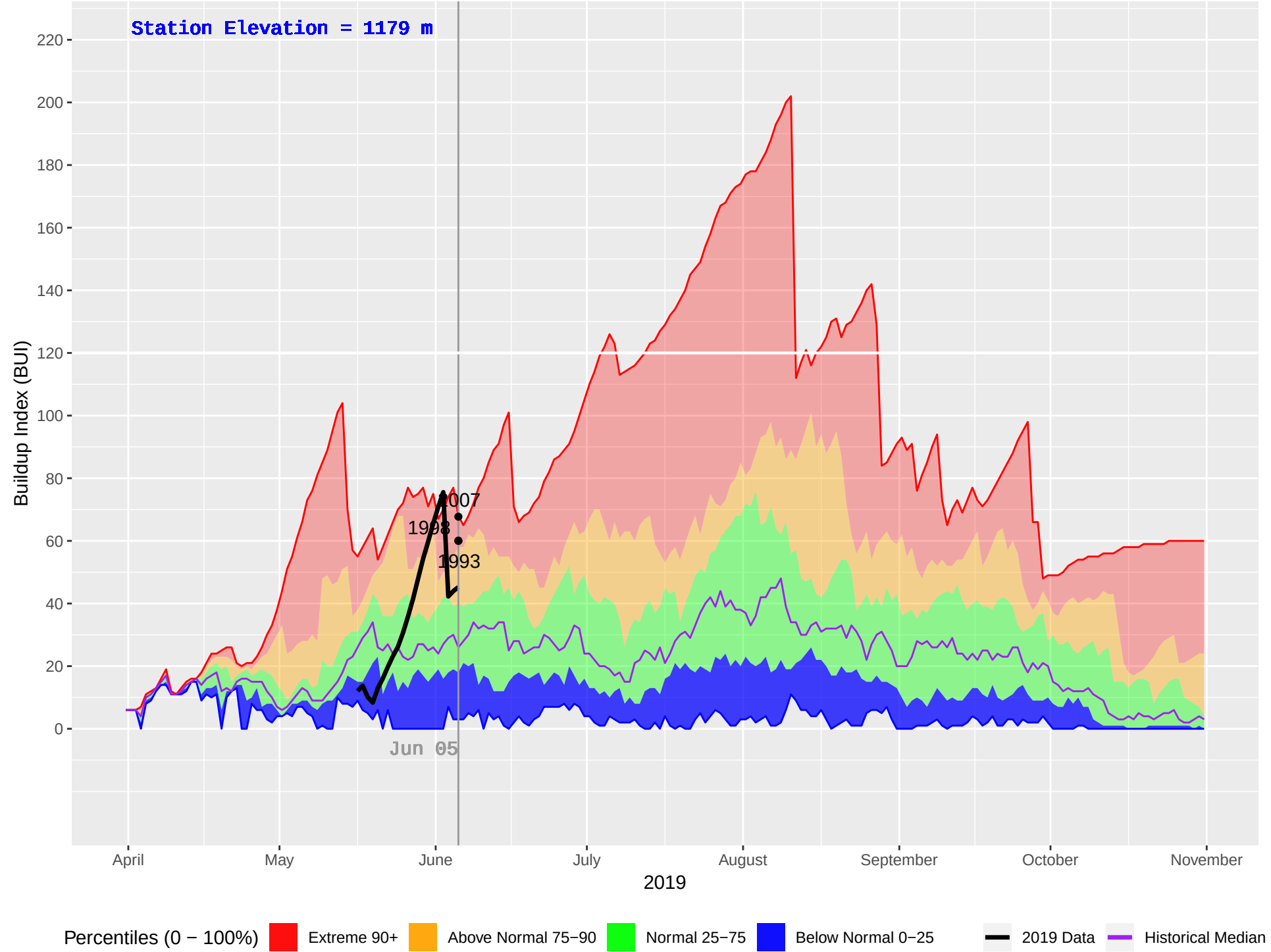
HOLMES (201) : Historical (1987–2018), Current (2019) Daily Buildup Index (BUI)
