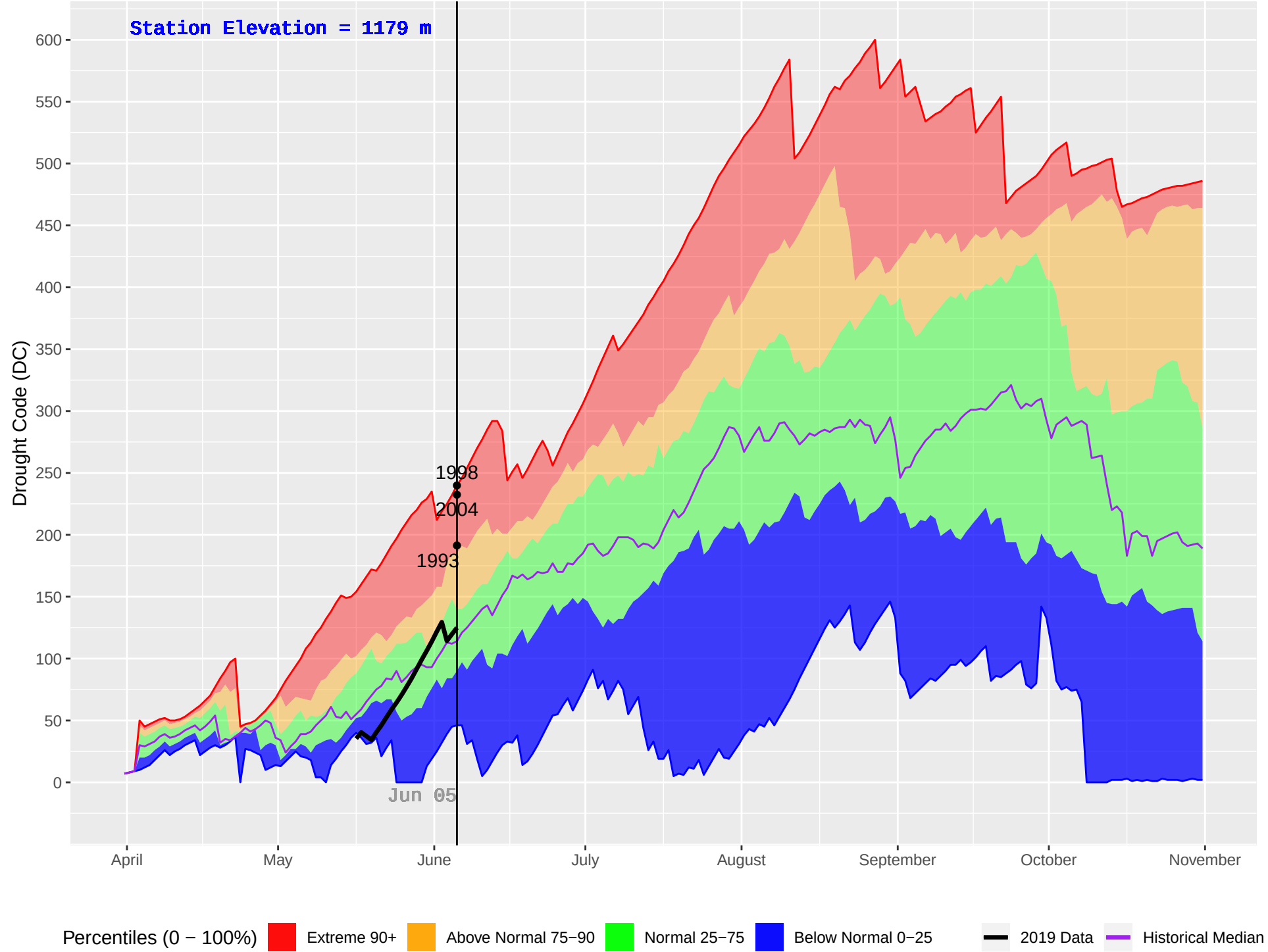
HOLMES (201) : Historical (1987–2018) and Current (2019) Daily Drought Code (DC)
