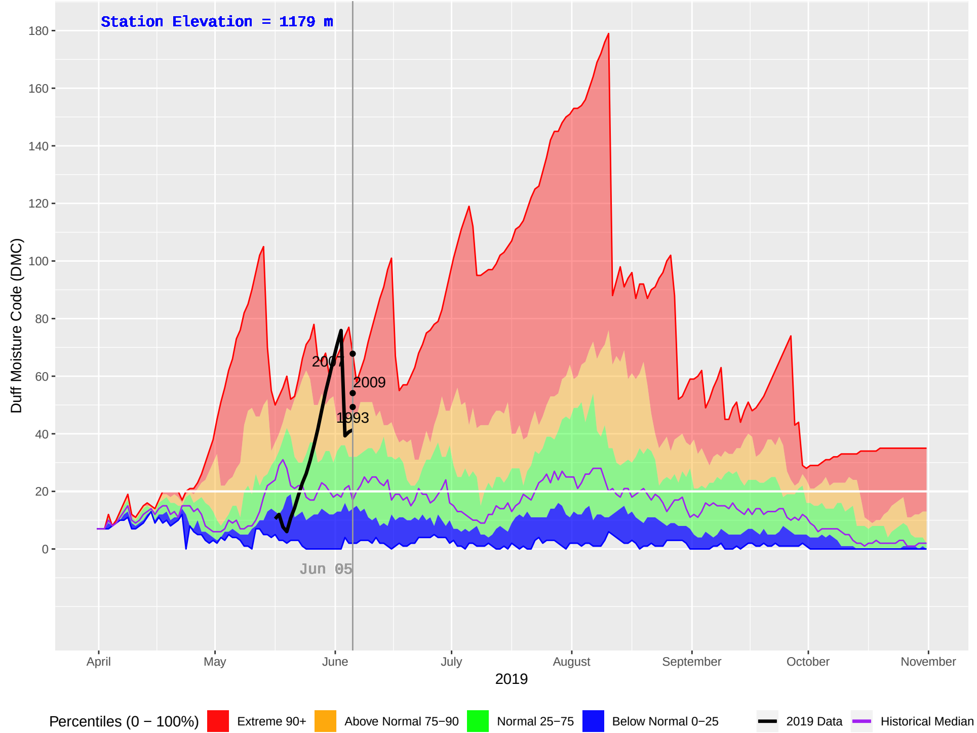
HOLMES (201) : Historical (1987–2018), Current (2019) Daily Duff Moisture Code (DMC)
