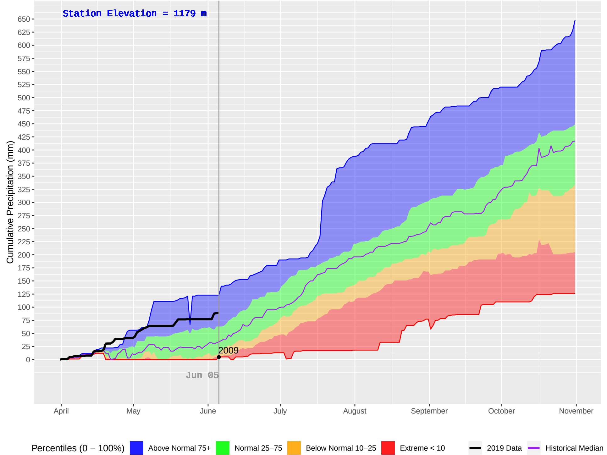
HOLMES (201) : Historical (1987–2018), Current (2019) Daily Cumulative Precipitation
