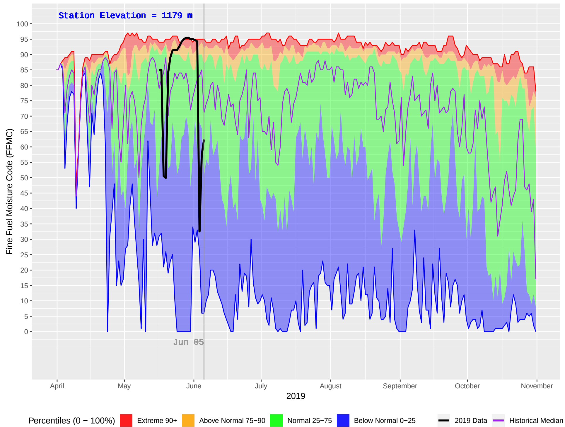
HOLMES (201) : Historical (1987–2018) and Current (2019) Daily Fine Fuel Moisture Code (FFMC)
